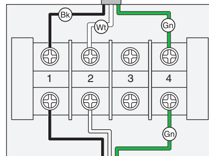
POWER CONNECTION BOX
